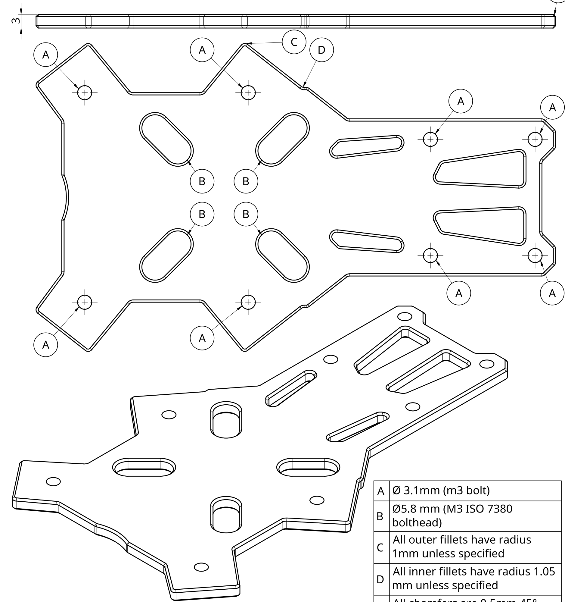
Bottom plate (3mm thickness)
