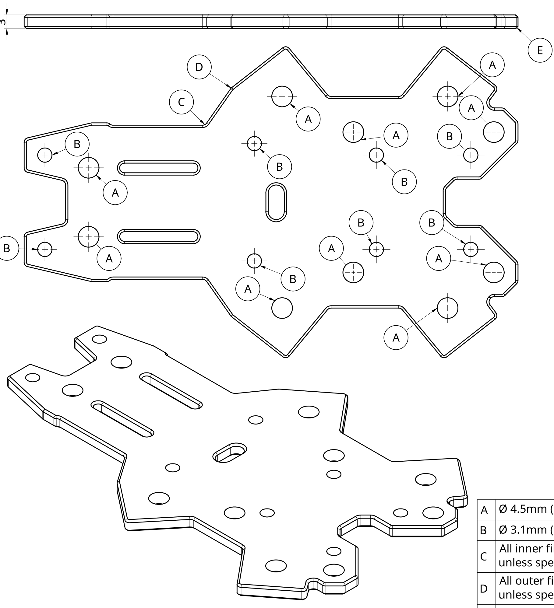
Middle plate (3mm thickness)
