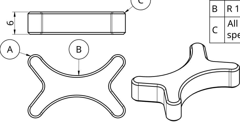
Cross (6mm thickness)
