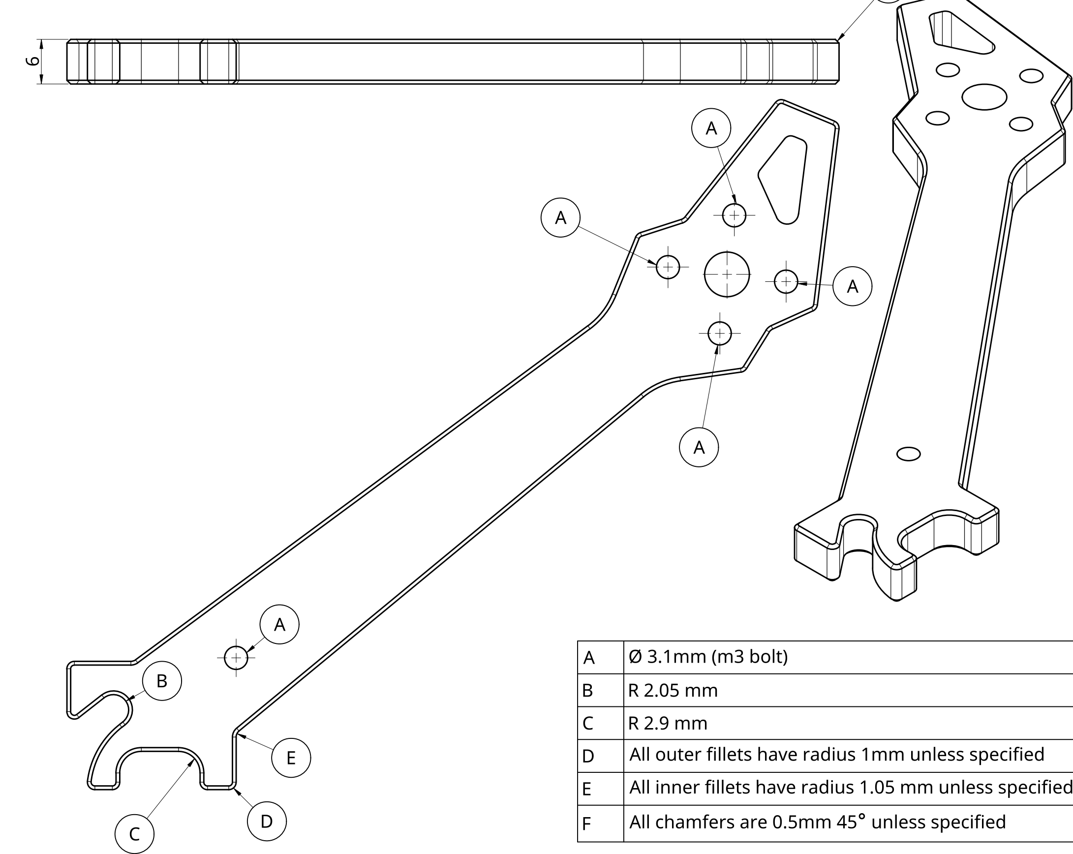
Arm (6mm thickness)
