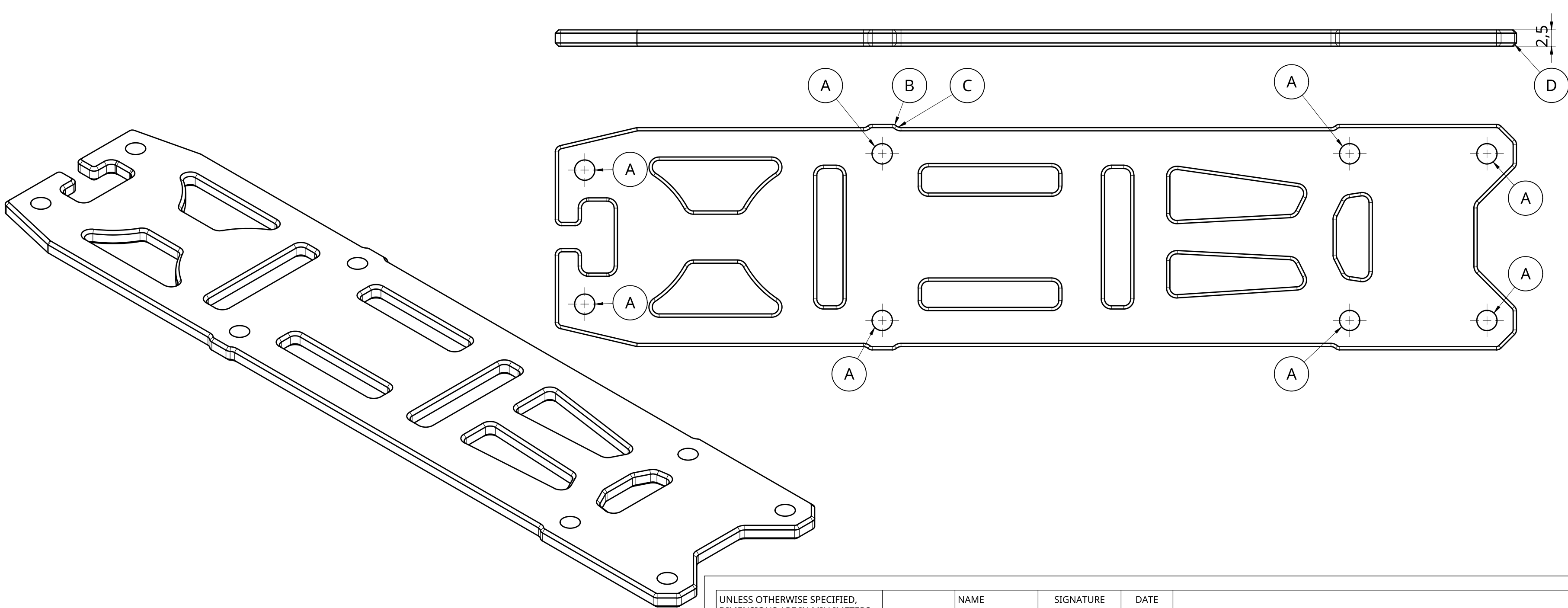
Top plate (2.5mm thickness)
