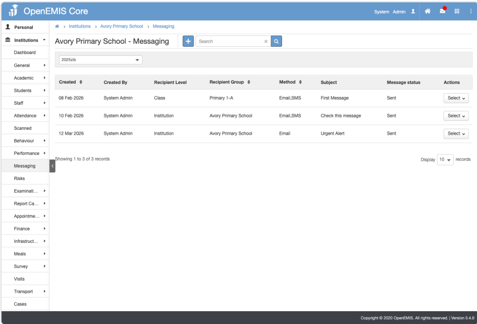
messaging-list screenshot
