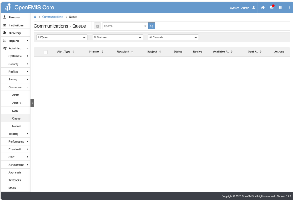
alert-queue screenshot
