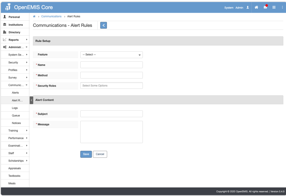
alert-rule-add screenshot
