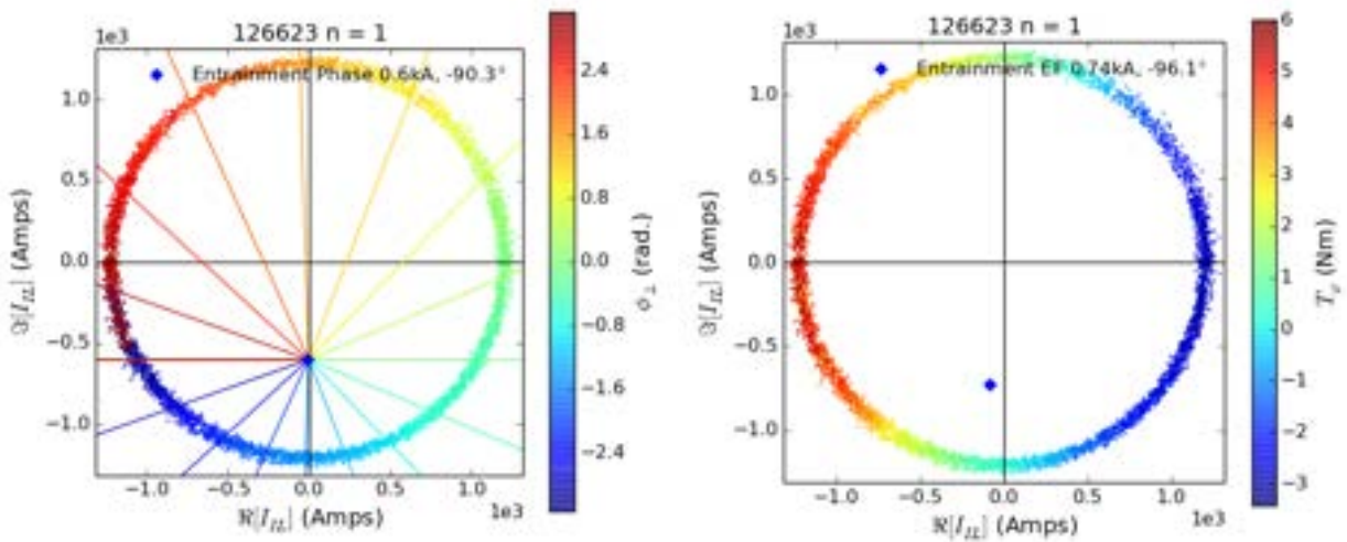
Figure 3.5: Left: The measured phase of the plasma field perpendicular to the LFS vessel midplane is indicated by by color and plotted on the trajectory of the complex I-coil current \mathbf{I}_{IL} . The optimal EFC (blue diamond) is determined by a least-squares fit to Eq. (3.5), and solid contours of constant total EF phase, \angle \mathbf{I}_T , are shown for the fit. Right: The measured EM torque plotted on the rotating trajectory of the complex coil current. The optimal EFC (blue diamond) is determined by a least-squares fit to Eq. (3.7). Both plots use data from between 1900 and 4900ms in shot 126623. In each case, the x and y axes are the real and imaginary components of the lower I-coil current rotated by 120 degrees to translate to an effective mid-plane phase for consistency with Ref. [83].
