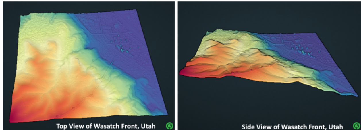
Figure 8: A 3D point cloud of the Wasatch Front in Salt Lake City, Utah, colored by elevation with purple as low elevation and red as high elevation. (left) The top view and (right) side view shows the elevation variations across the landscape. This shows mountains in warmer tones (orange-red) and the valley and city in cooler tones (blue). [6]
