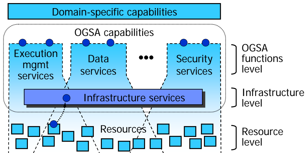
Figure 1: Levels of management in OGSA
