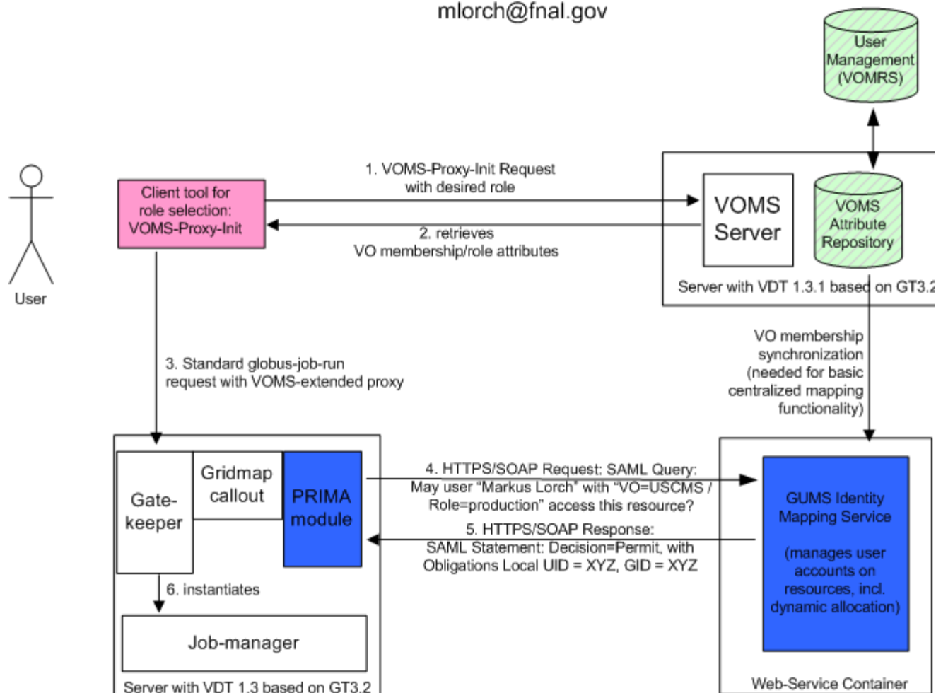
Figure 1 - Privilege Architecture Overview - Grid User Mapping Usecase
