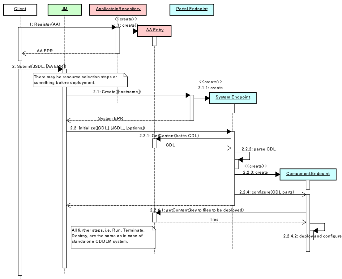
Figure 3-5 Possible Interaction with CDDL (example)
