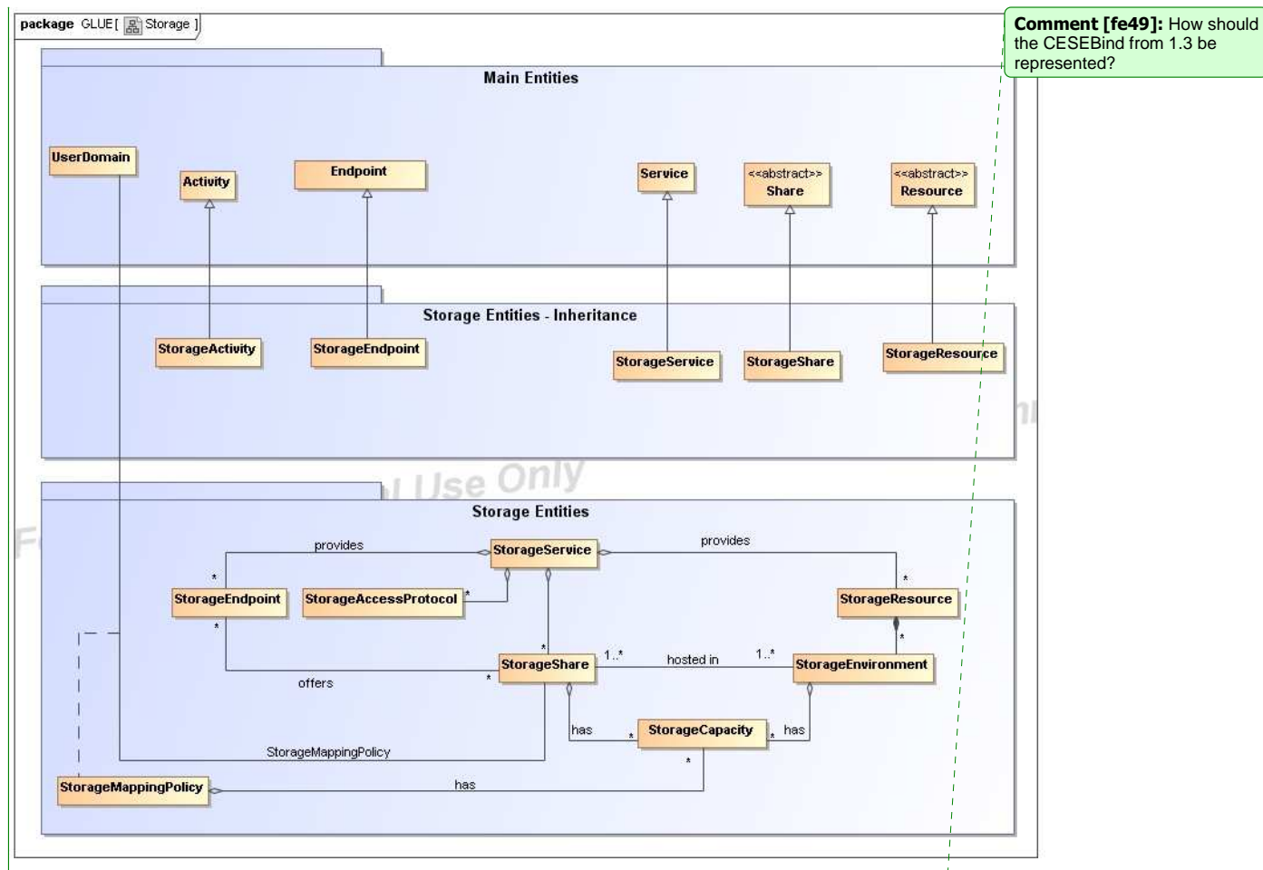
Figure 4 Entities and relationships for the Storage Element model
