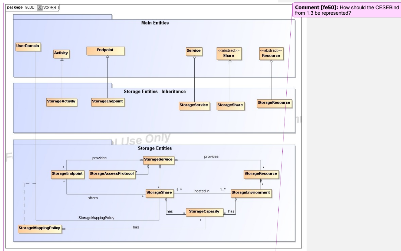
Figure 4 Entities and relationships for the Storage Element model
