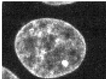
B XZ · central body reviewed through depth
