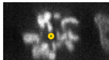
C YZ · one assigned centre, unresolved multi-lobed identity
