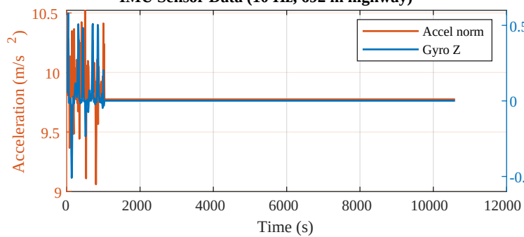
IMU Sensor Data (10 Hz, 692 m highway)
