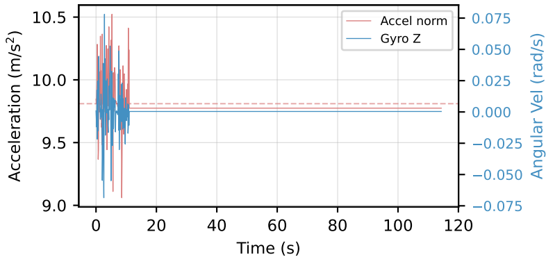
IMU Sensor Data (10 Hz, 692 m highway)
