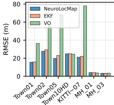
(a) RMSE Comparison
