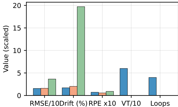
(a) Town01 Metrics (517 m, 5000 frames)
