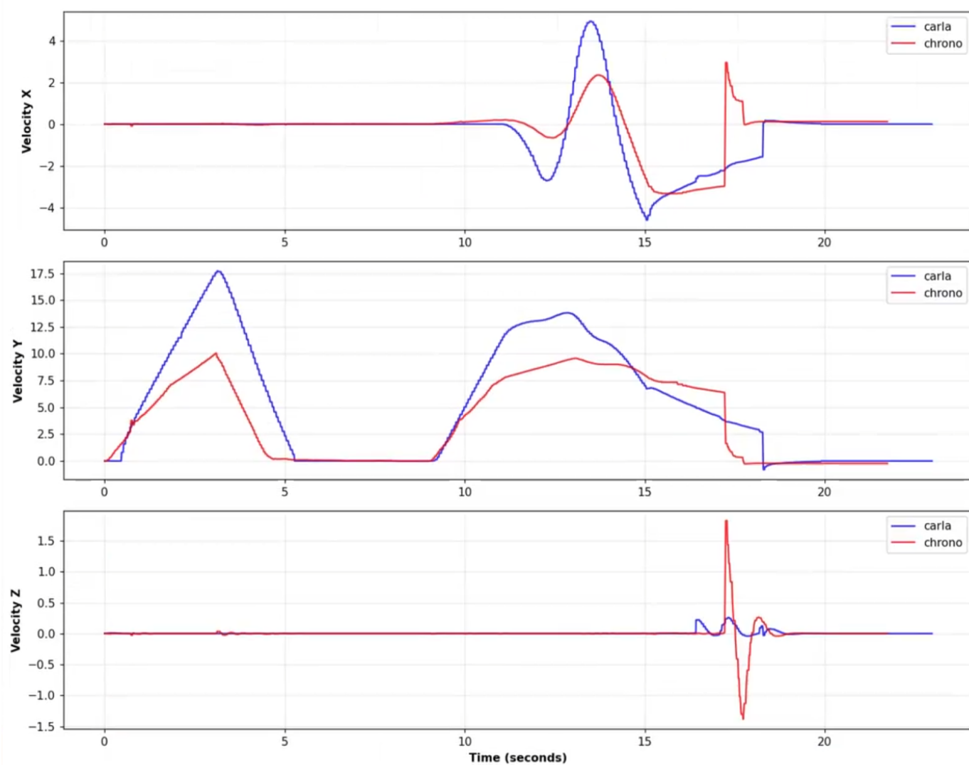
IMU Data Comparison - Velocity
