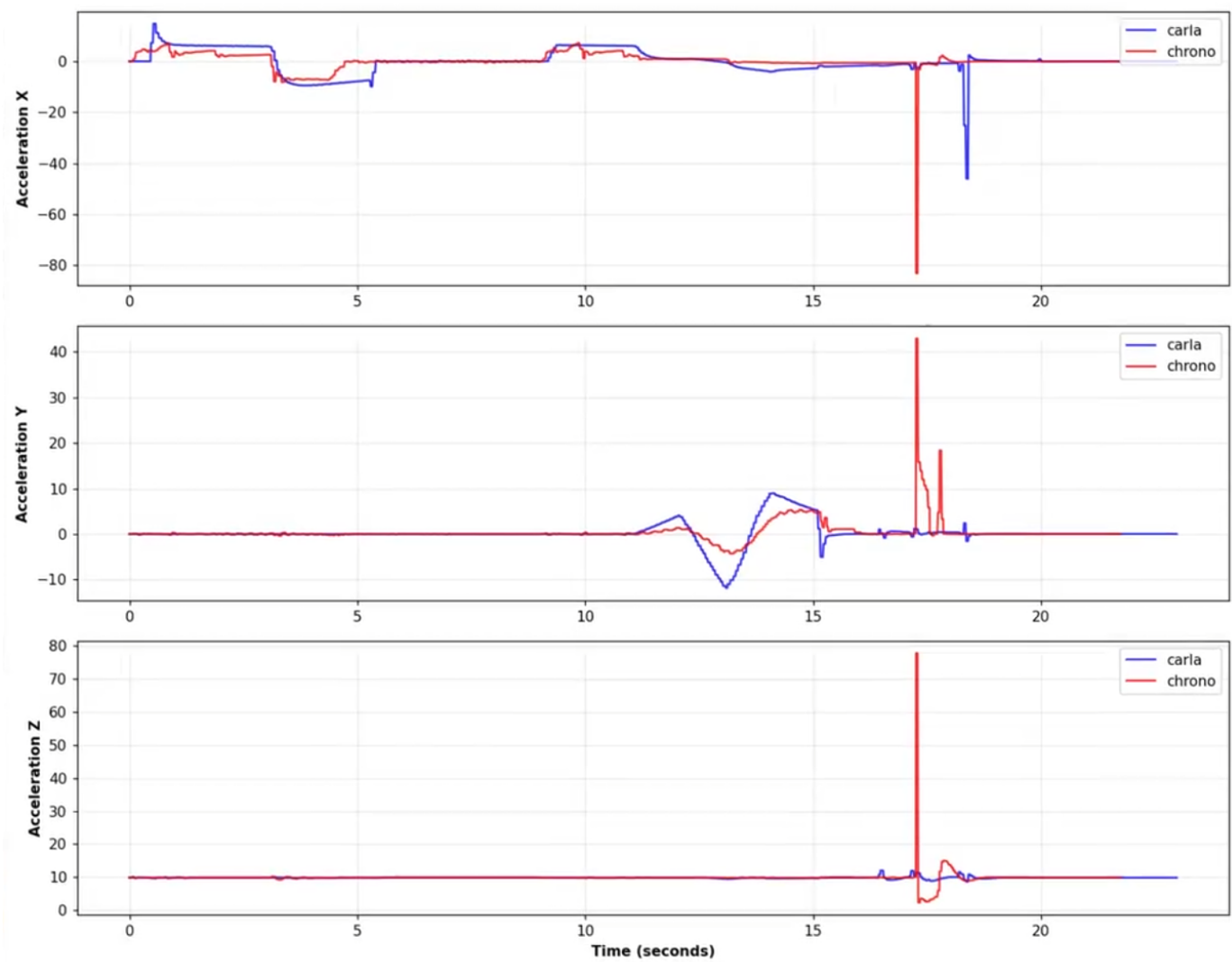
IMU Data Comparison - Acceleration
