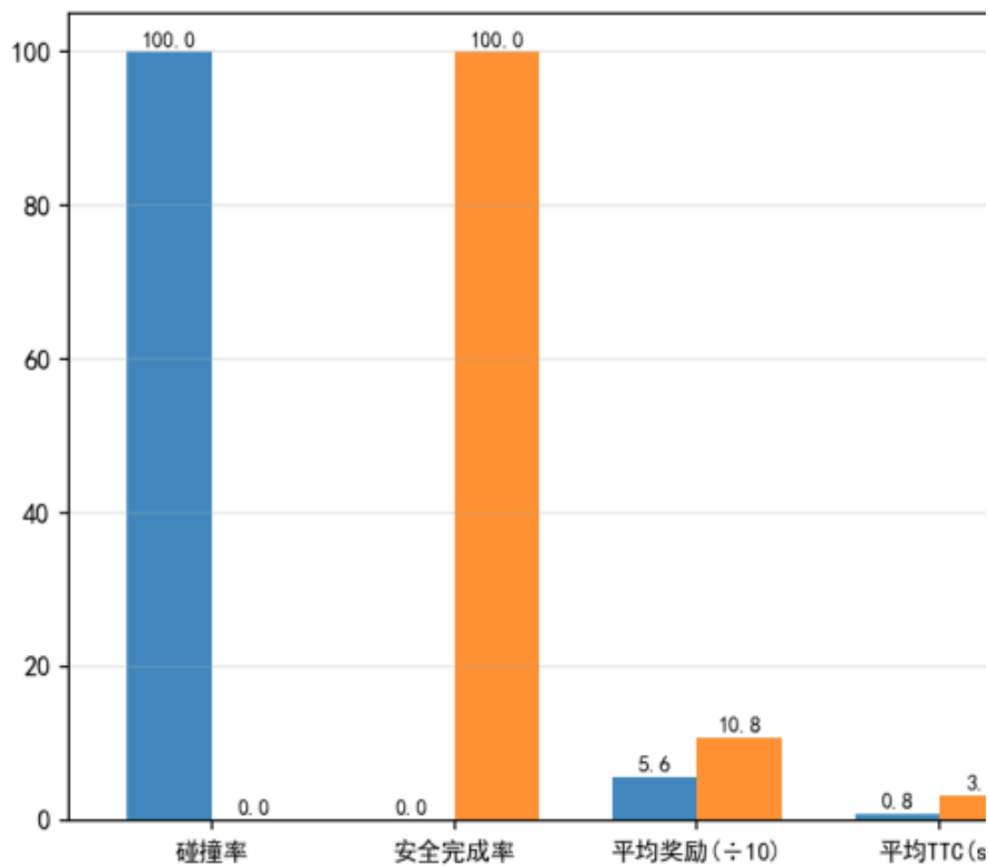
Evaluation Metrics: Attention-DQN vs Smooth-PP0
