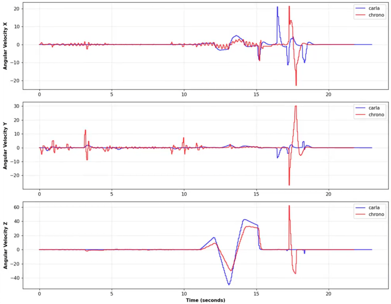
IMU Data Comparison - Angular Velocity
