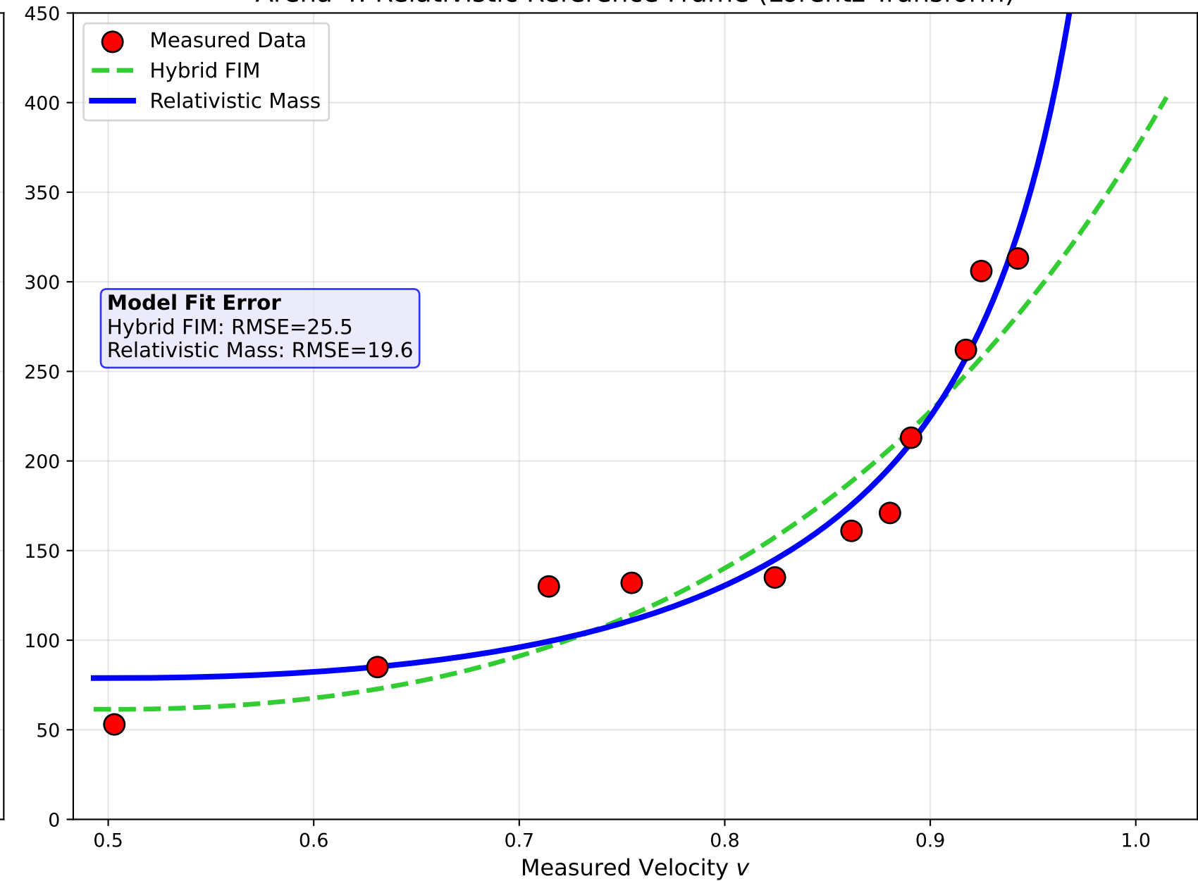
Arena 4: Relativistic Reference Frame (Lorentz Transform)
