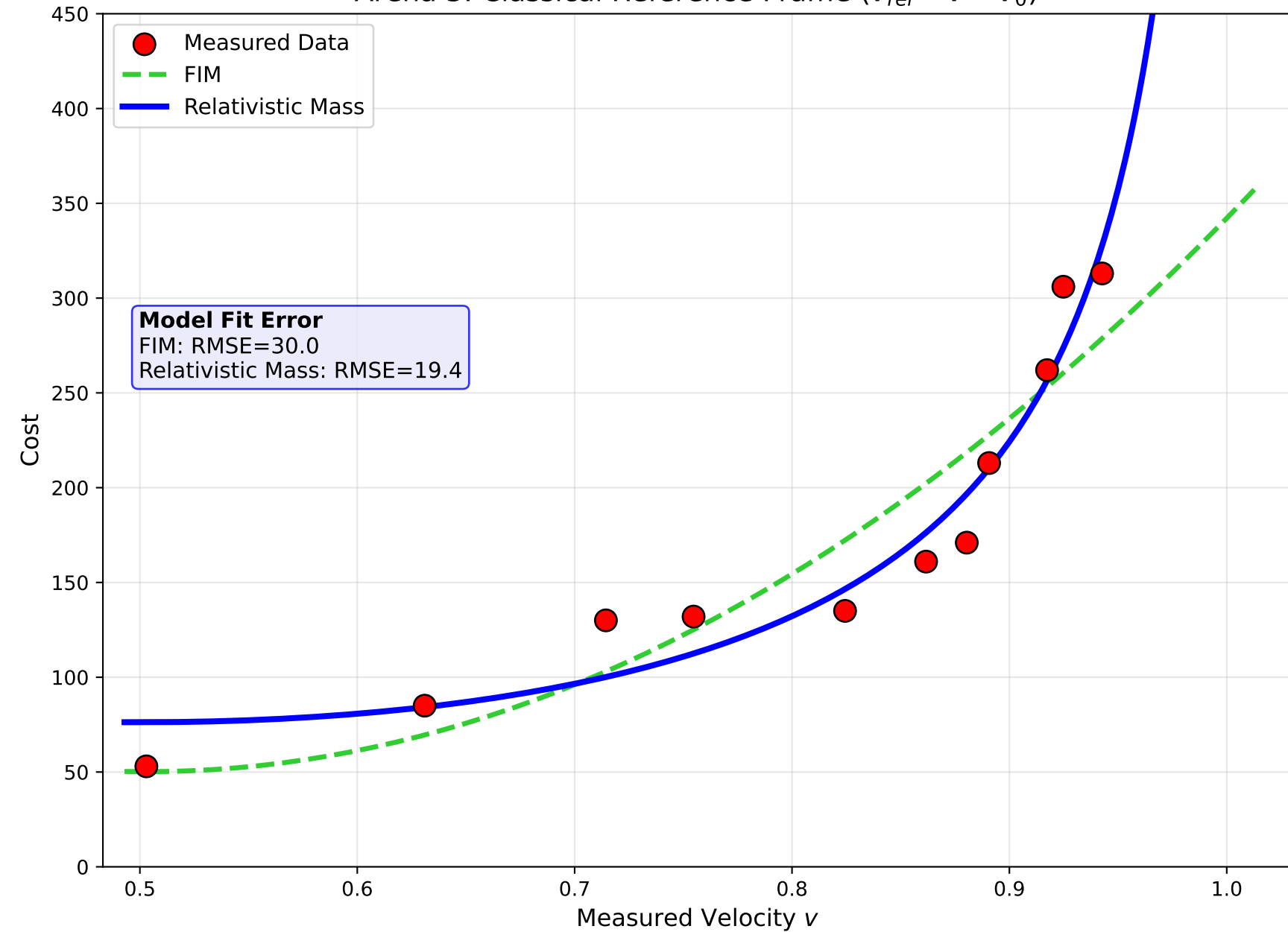
Arena 3: Classical Reference Frame ( v_{rel} = v - v_0 )
