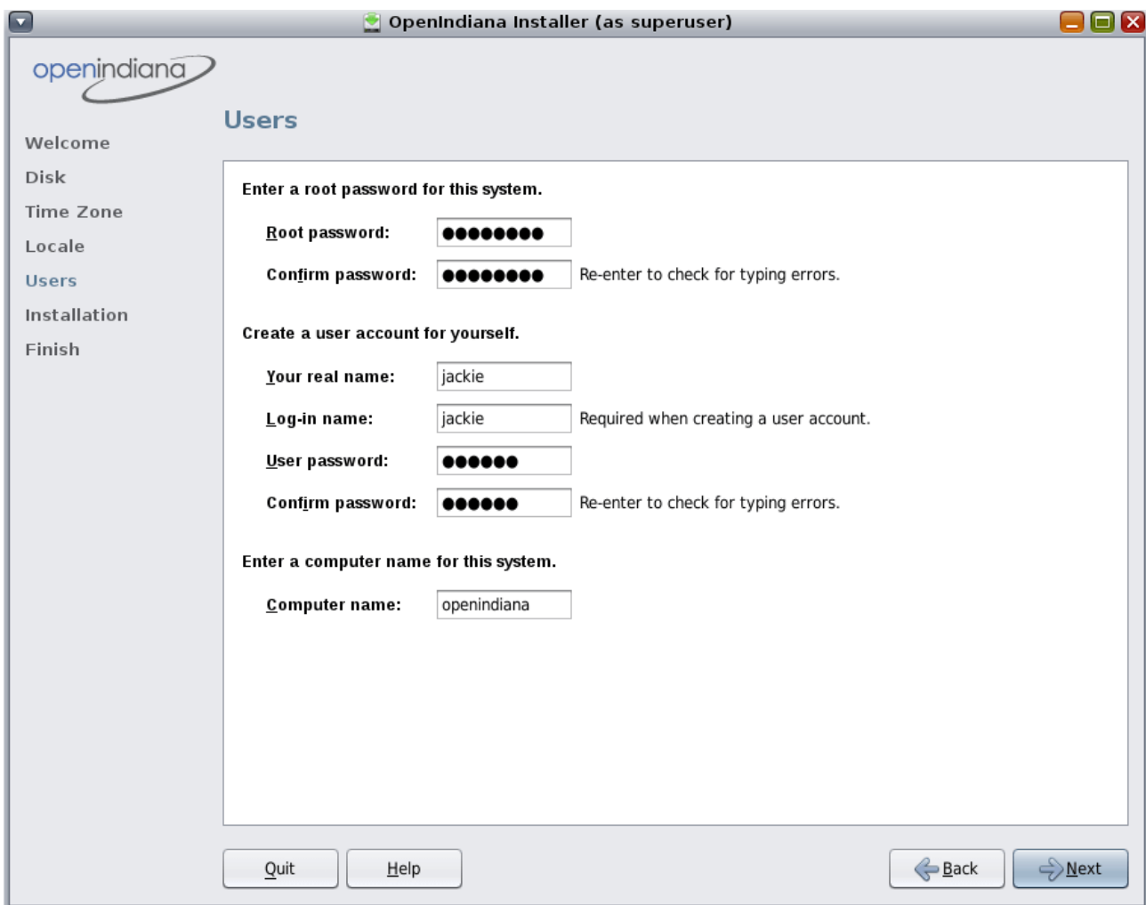
Figure 11: Users
