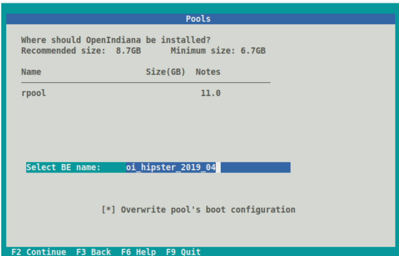
Figure 33: Pools Screen
