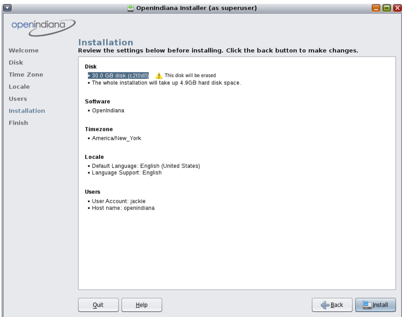
Figure 12: Installation summary
