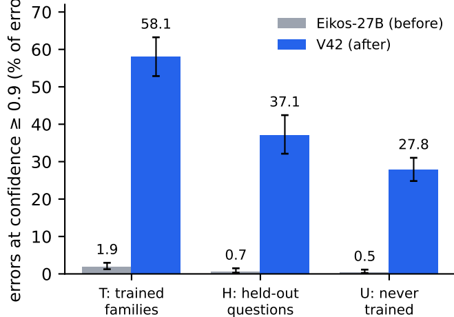
(b) errors made with confidence
