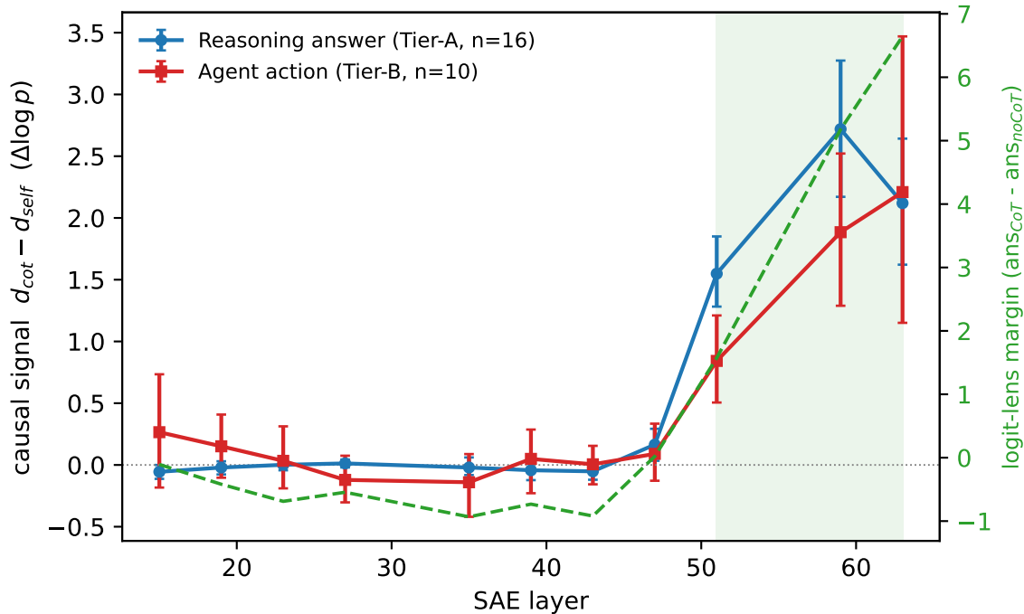
The late channel: causal CoT content concentrates in L51--63
