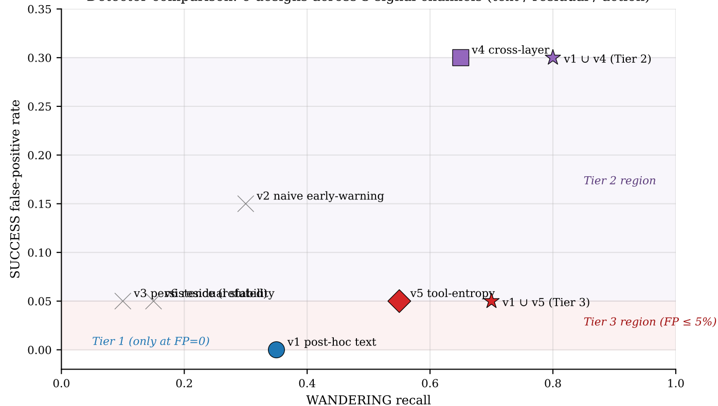
Detector comparison: 6 designs across 3 signal channels (text / residual / action)
