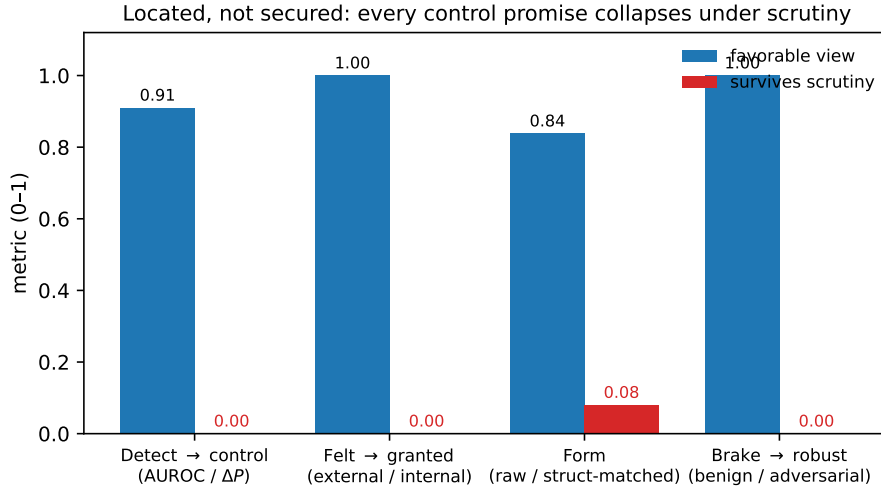
Figure 1: Four of the five limits, as matched pairs. Each control promise (blue, the favorable view) collapses when the right control is applied (red): detection AUROC 0.91 vs control effect \approx 0 ; an external check catching the realistic over-reach vs the internal monitor (0); raw AUROC 0.838 vs structure-matched 0.08; benign brake suppression vs adversarial robustness ( 1 - \text{ASR} ). The fifth limit (intervention easy where unneeded) is qualitative and not plotted.
