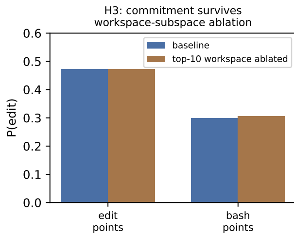
Figure 4: H3. Ablating the top-10 verbalizable directions at the decision point leaves the commitment differential intact.
