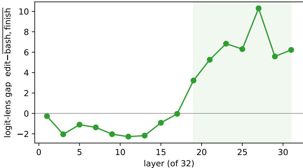
Mistral-7B (diff. family): commit decision emerges late
