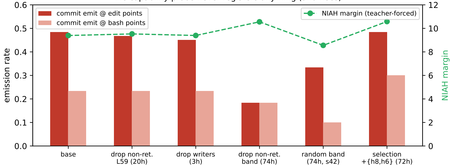
The two-sided audit: commitment collapses under the criterion's band ablation; the capability probe never registers anything (and rises)
