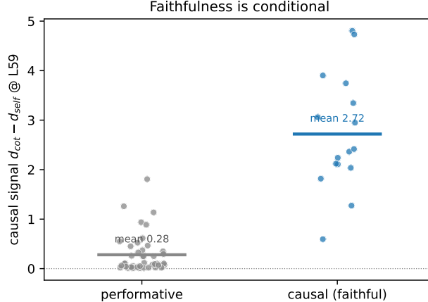
Figure 2: Conditional faithfulness. Causal signal at L59 per item, split by whether the CoT changes the answer. Already-correct-without-CoT ( n=44 ): CoT features non-causal (mean +0.28 ). CoT flips the answer ( n=16 ): features strongly recover it (mean +2.72 ). Bars are group means.
