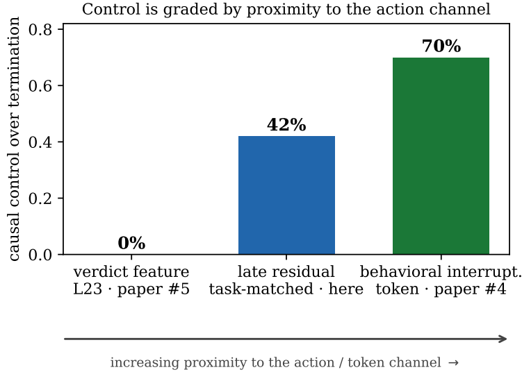
Figure 3: The graded law. Causal control over termination rises with proximity to the action channel: null at the verdict feature (paper #5), partial at the late task-matched residual (this work), dominant at the behavioral/token channel (paper #4). The three values come from three arc experiments with different baselines and n ; the ordering , not the exact heights, is the claim.
