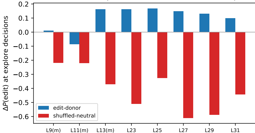
Mistral-7B writability: edit-donor writes, random vector destroys
