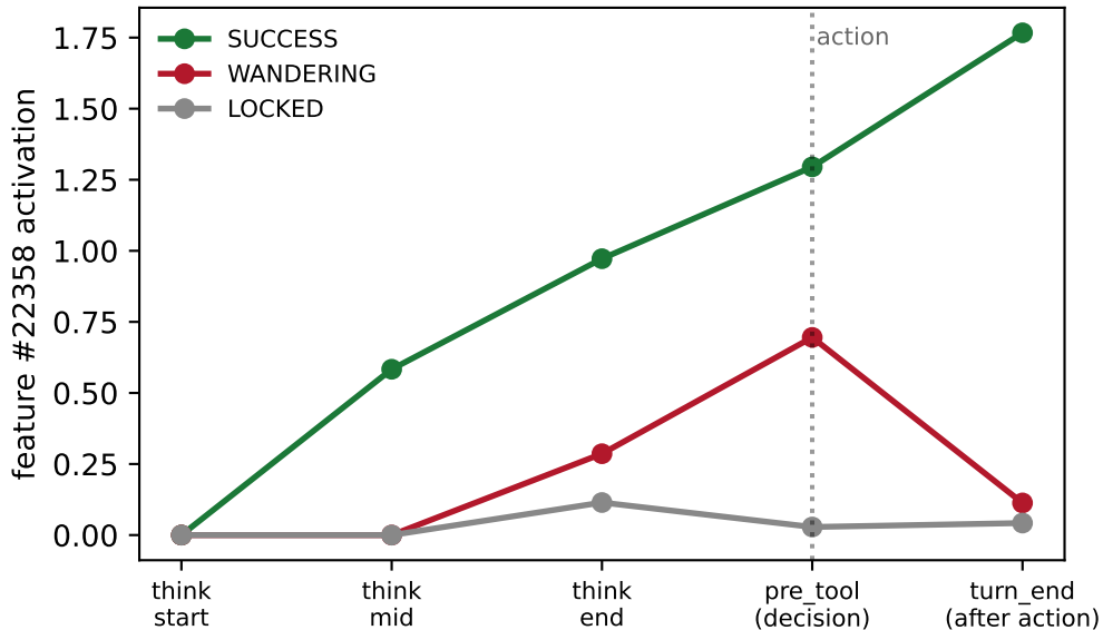
Verdict feature over the final turn
