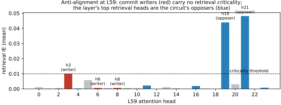
Figure 1: Retrieval importance (receiver IE, mean over 12 pairs) for all 24 heads of L59. The commit writers (red) sit at the floor; the layer’s strongest retrieval heads (blue) are the commitment circuit’s opposers.
