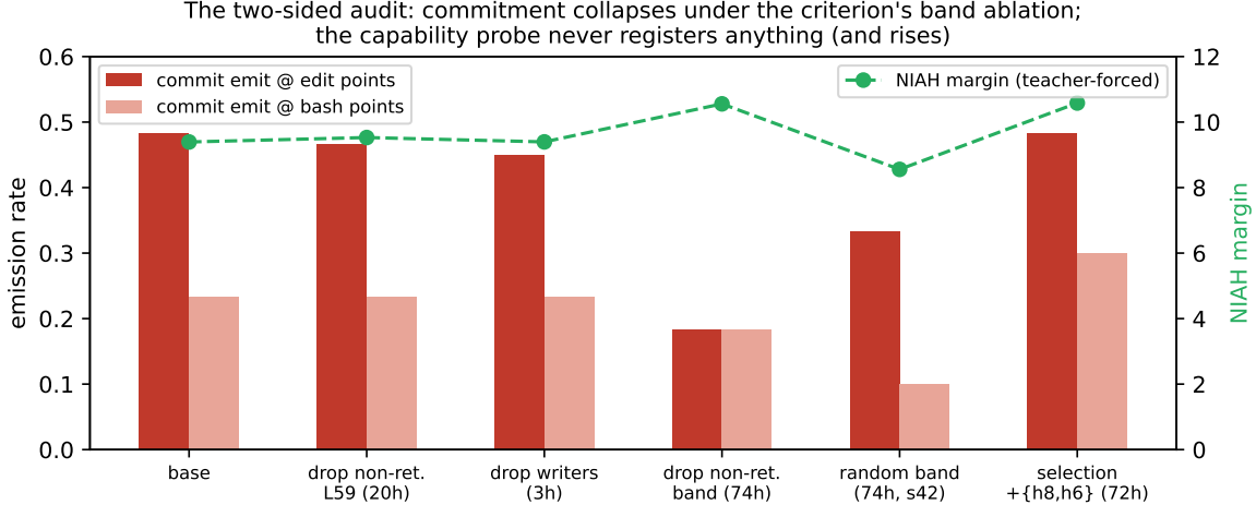
Figure 2: The two-sided audit across conditions: commitment emission (bars, left axis) versus the teacher-forced NIAH margin (green, right axis). Only the band-scope ablation of the criterion’s non-retained heads collapses commitment — and the capability probe’s margin rises .
