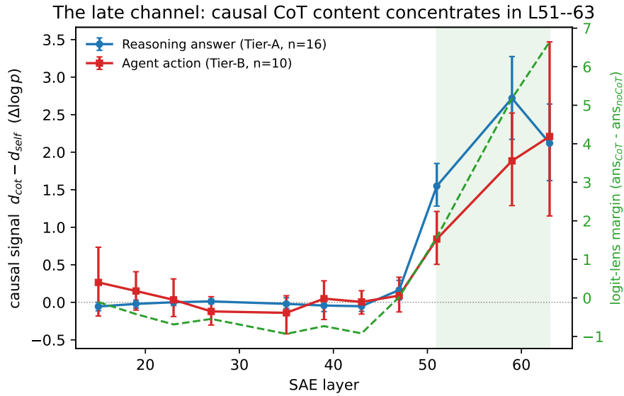
Figure 3: The late channel. Solid (left axis): causal patch signal d_{\text{cot}} - d_{\text{self}} per SAE layer for the reasoned answer (Tier-A) and agent action (Tier-B), bootstrap 95% CIs. Dashed (right axis): the logit-lens consolidation margin (§6). Both are \approx 0 or negative through mid layers and concentrate in L51–63 (shaded).
