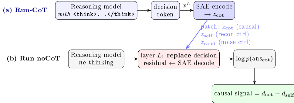
Figure 1: The causal-patch test. (a) Run-CoT produces the decision state, encoded to SAE features z_{cot} . (b) Run-noCoT is forced to the same answer slot; at SAE layer L we replace the decision-token residual with the SAE decode of z_{cot} and read \log p of the CoT answer. Patching z_{cot} gives the causal effect; z_{self} (the no-CoT features’ own reconstruction) controls for SAE error; z_{rand} is the noise baseline. Reported signal = d_{cot} - d_{self} .
