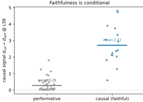
Figure 2: Conditional faithfulness. Causal signal at L59 per item, split by whether the CoT changes the answer. Already-correct-without-CoT ( n=44 ): CoT features non-causal (mean +0.28). CoT flips the answer ( n=16 ): features strongly recover it (mean +2.72). Bars are group means.
