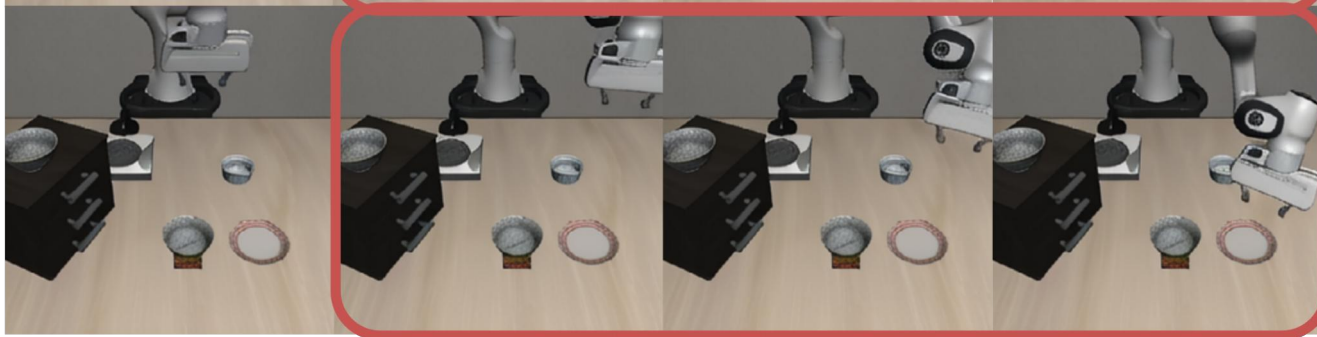
Ctrl-World
