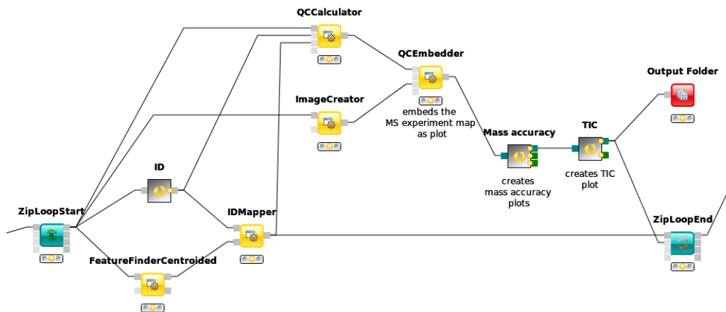
Figure 45: Basic QC setup within a LFQ workflow
