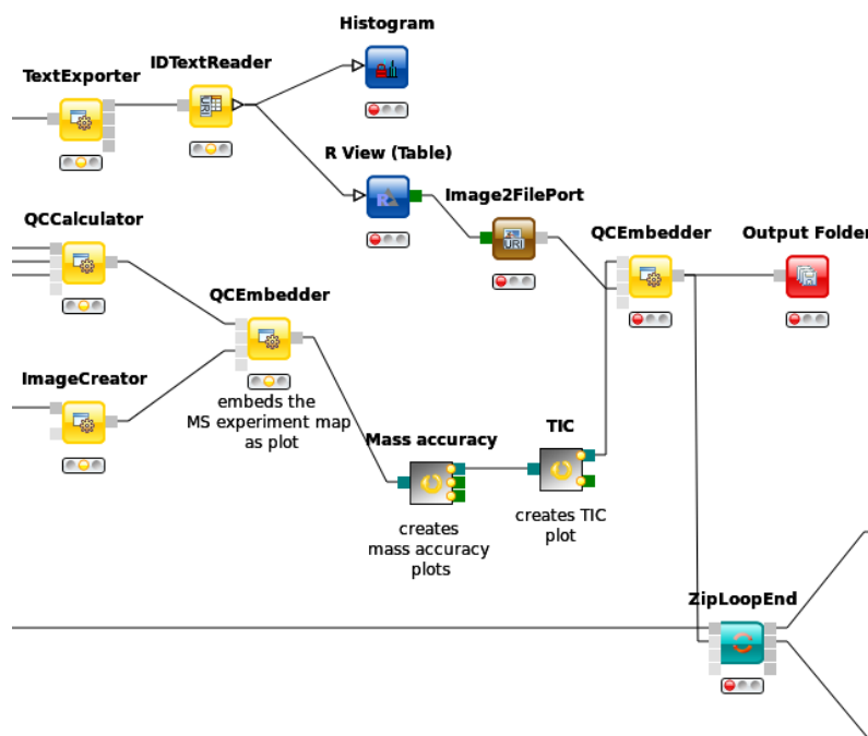
Figure 46: QC with new metric
