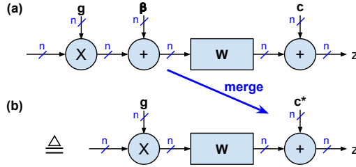
Figure 3: Elimination of bias \beta : (a) Before elimination with \beta between normalization weights \mathbf{g} and linear layer. (b) Optimized version with new bias term \mathbf{c}^* = \mathbf{c} + \beta\mathbf{W} at the output.
