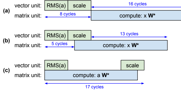
Figure 8: Example timing diagrams. (a) Sequential: matrix unit idles 8 cycles. (b) Partial overlap with interleaved scaling and vector-matrix multiplication. (c) FlashNorm : vector-matrix multiply and RMS run fully in parallel.
