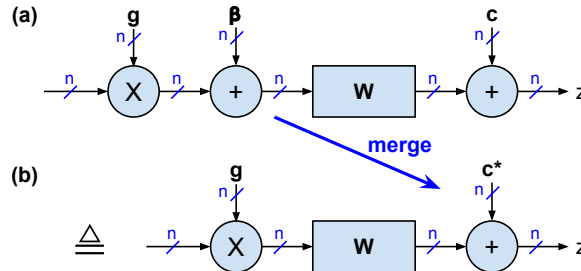
Figure 3: Elimination of bias \beta : (a) Before elimination with \beta between normalization weights g and linear layer. (b) Optimized version with new bias term \mathbf{c}^* = \mathbf{c} + \beta\mathbf{W} at the output.
