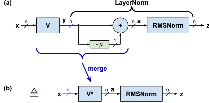
Figure 8: Elimination of mean centering: (a) Original weight matrix \mathbf{V} followed by mean centering. (b) Optimized version where the mean centering is merged into the modified weight matrix \mathbf{V}^* .
