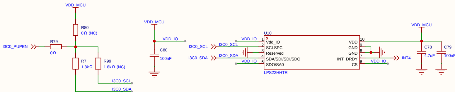
I3C Pressure Sensor
