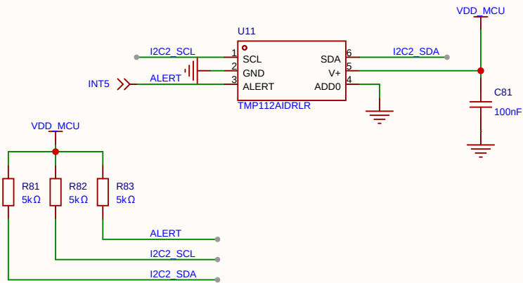
I2C Temperature Sensor
