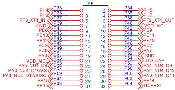
HEADER 2.54 16X2 male
