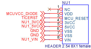
HEADER 2.54 8X1 female
