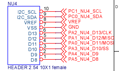
HEADER 2.54 10X1 female
