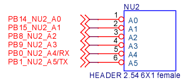
HEADER 2.54 6X1 female
