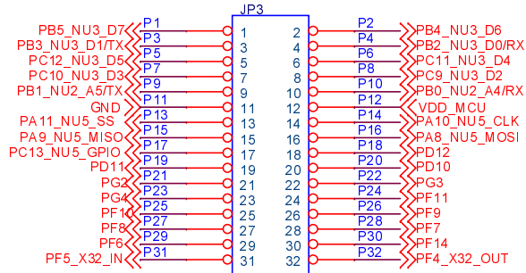
HEADER 2.54 16X2 male
