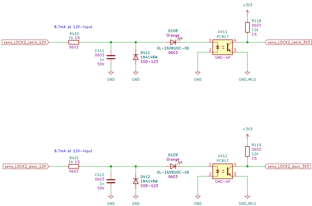
Lock2 sensors' processing circuits
