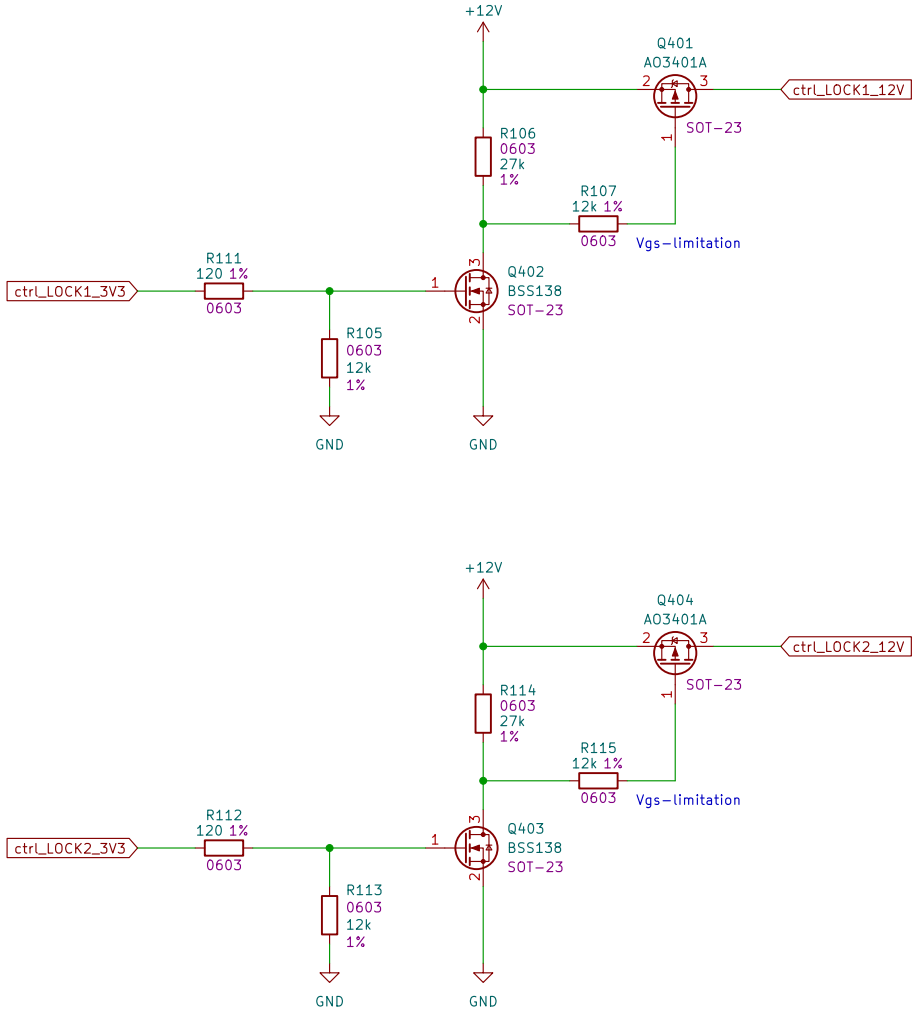
Locks' control circuits
