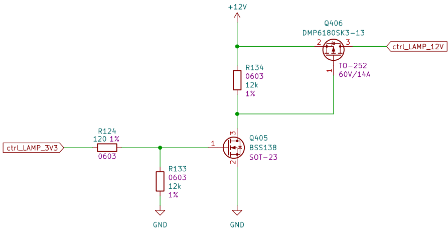
Lamp control circuit
