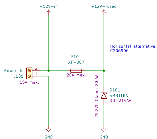
Overcurrent and overvoltage protection
