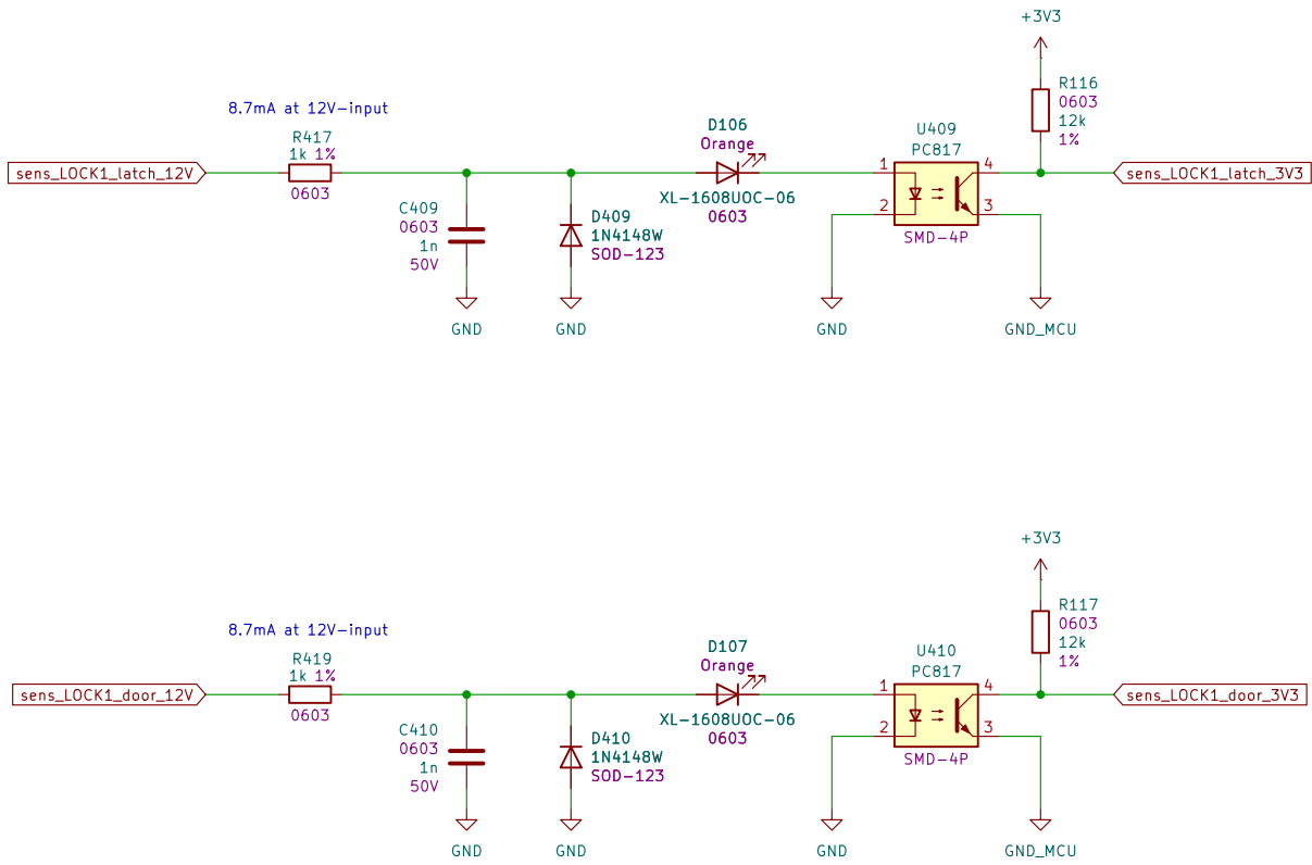
Lock1 sensors' processing circuits
