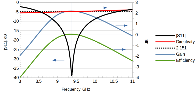
Figure 36: Far-field metrics.
