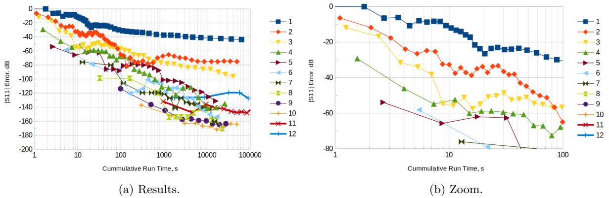
Figure 29: |S_{11}| error.
