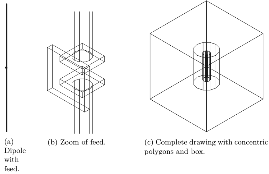
Figure 34: Dipole antenna.
