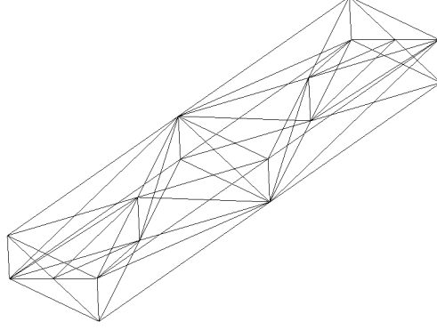
Figure 27: Initial mesh for the 100 mm long WR90 rectangular waveguide.
