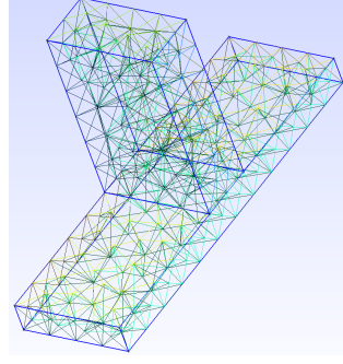
Figure 20: Mesh for the WR75 T-Junction.
