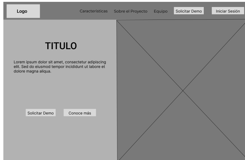
Figure 18: wireframe
