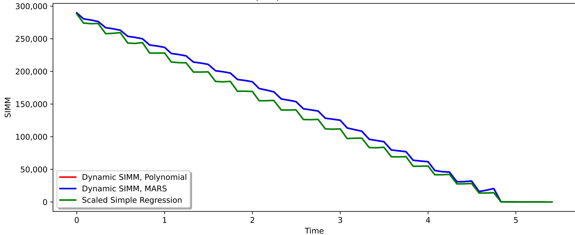
Swap Expected Discounted SIMM
