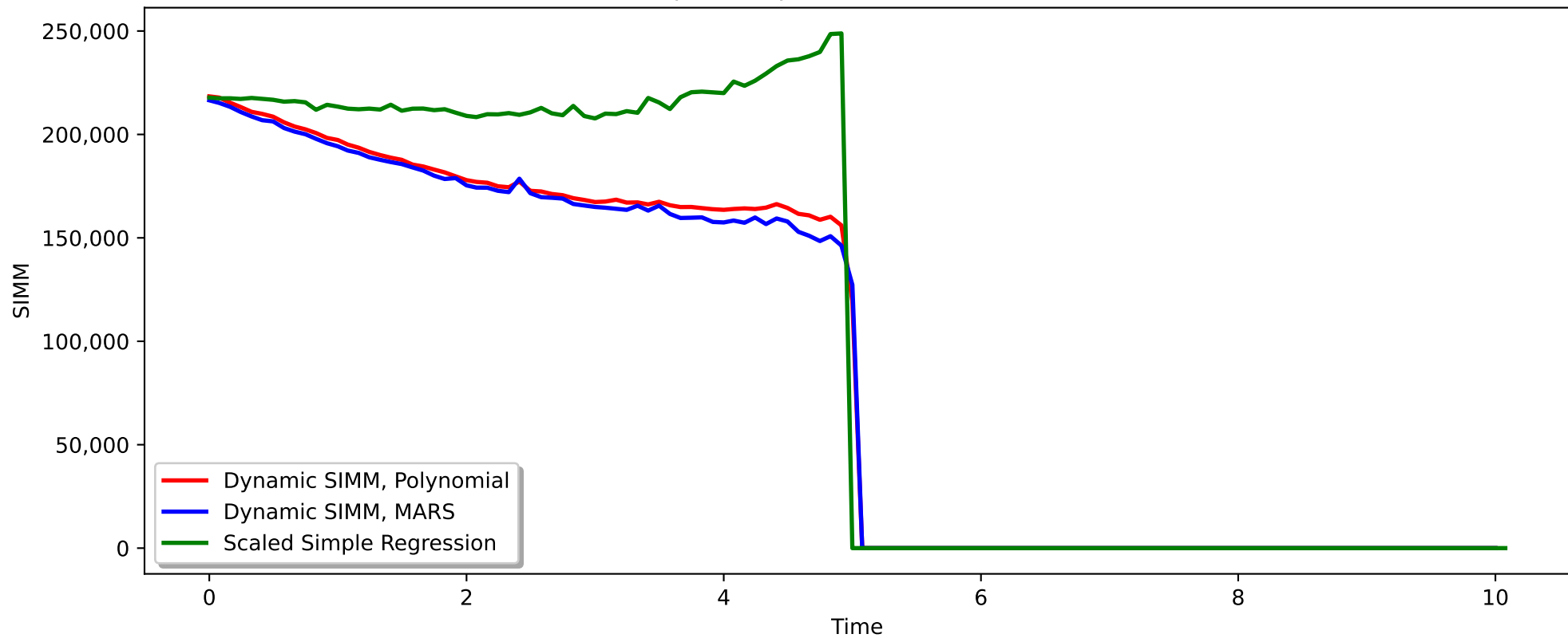
Swaption Expected Discounted SIMM
