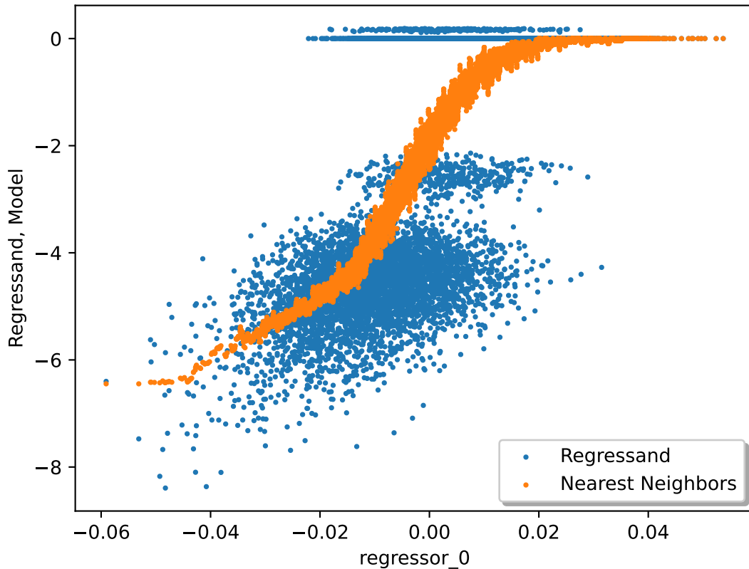
1e3 Bermudan: irDelta_EUR_5Y regression at time 4Y
