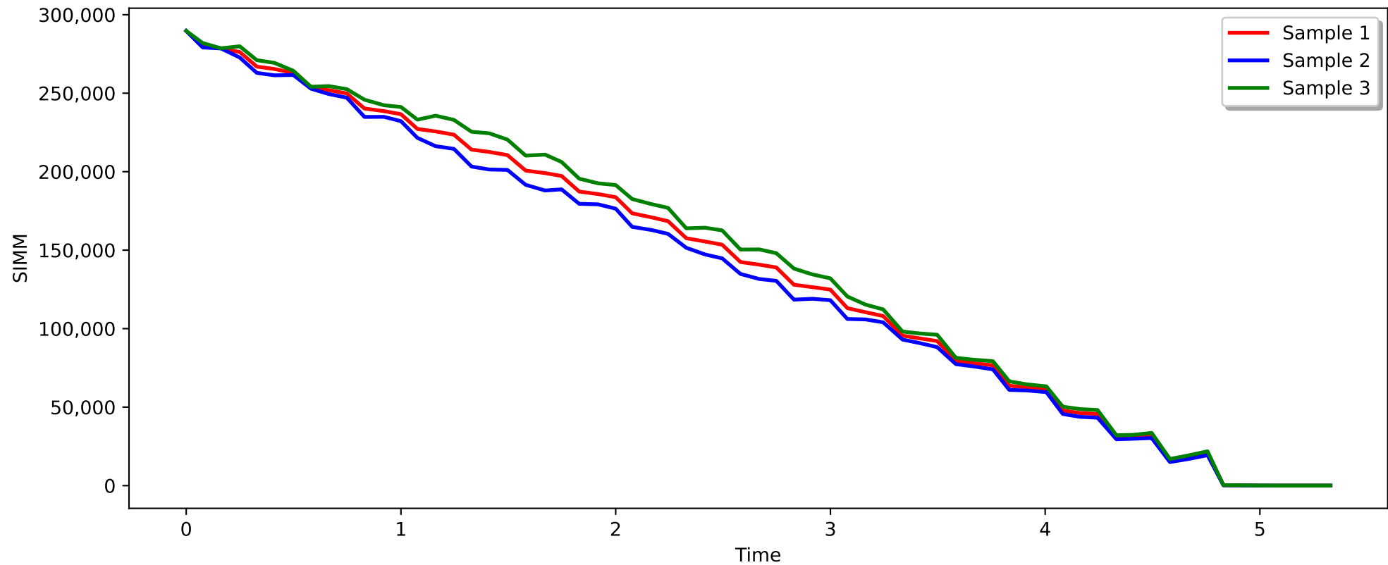
SIMM Evolution Pathwise
