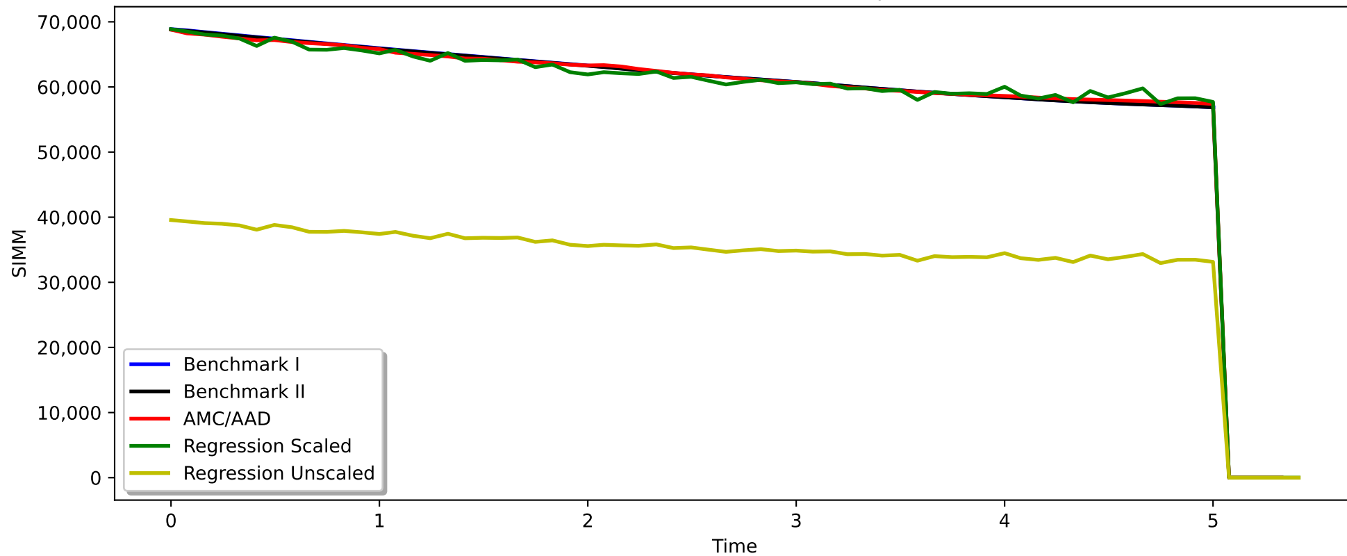
SIMM Evolution Pathwise, Sample 1
