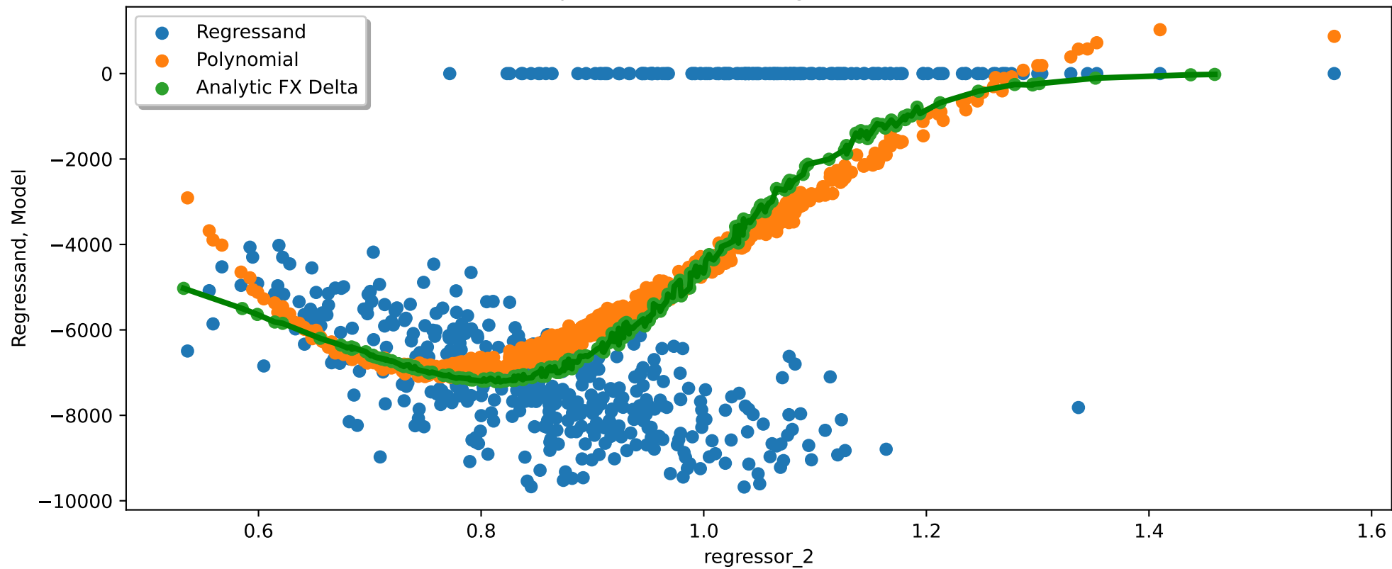
FX Option: fxDeltaUSD regression at time 3Y
