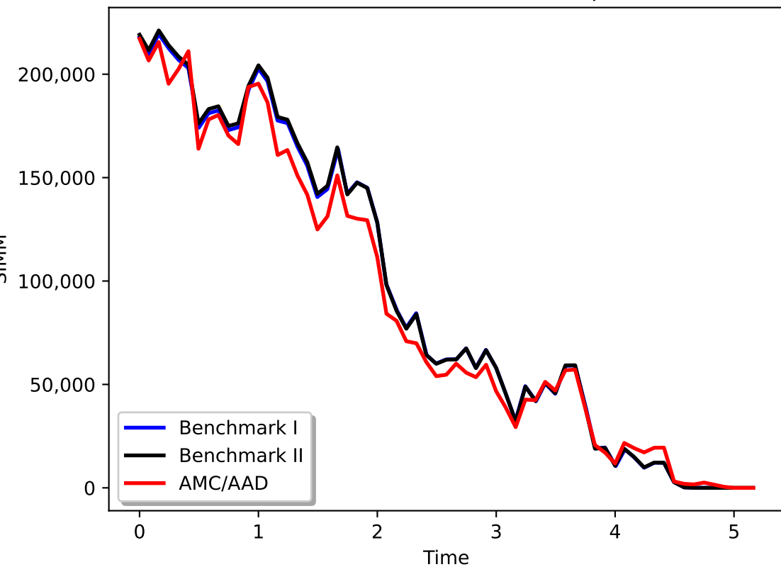
SIMM Evolution Pathwise, Sample 2
